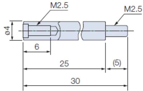
Extension spindle
